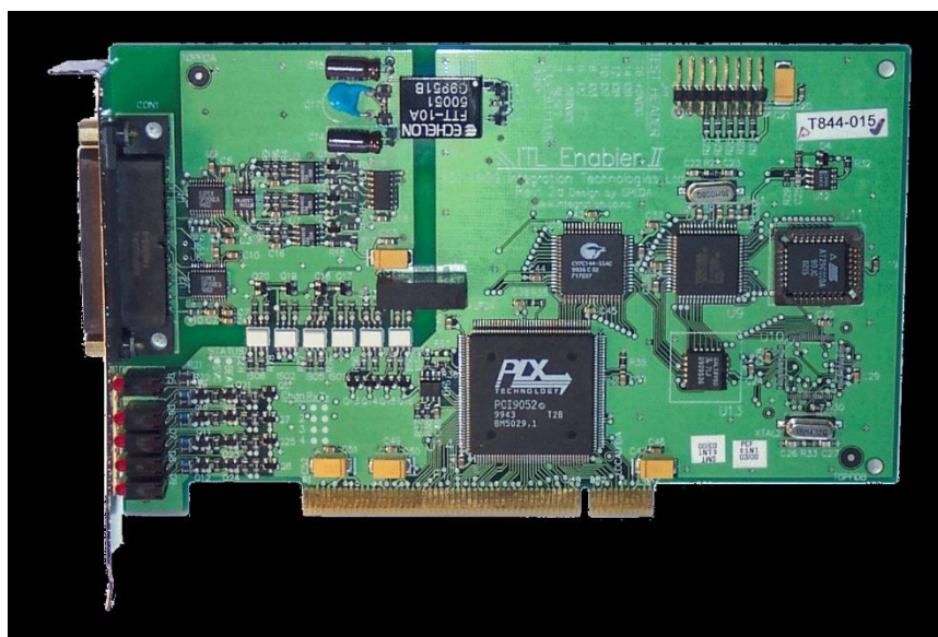
(b) Model Enabler 2 PCI Controller (The Pattern)
