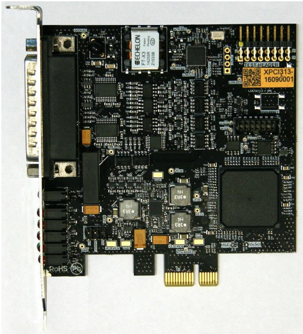
Model Enabler Express Controller (Variant 5)
