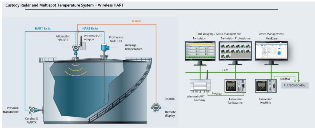
(c) Wireless Hart System Architecture
