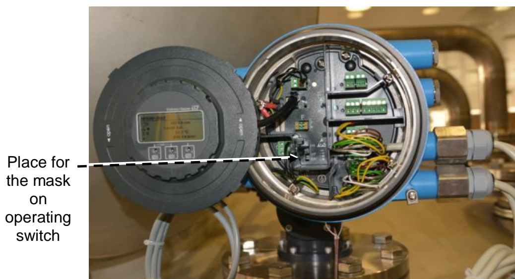
Typical Sealing of Operation Switch
