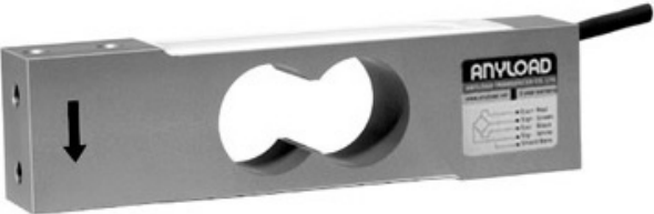
(l) ANYLOAD model 108TAUN
