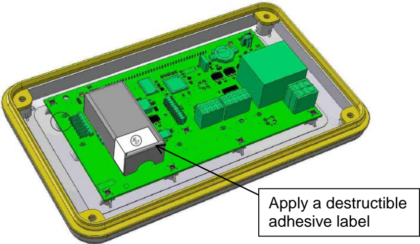
(b) Destructible Adhesive Label Sealing
