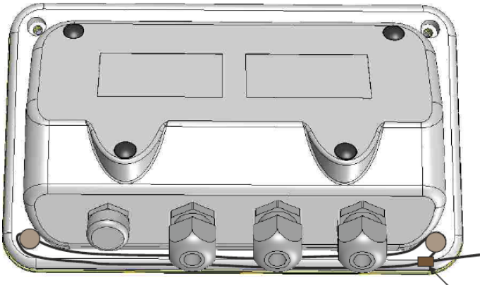
(a) Lead and Wire Type Sealing
