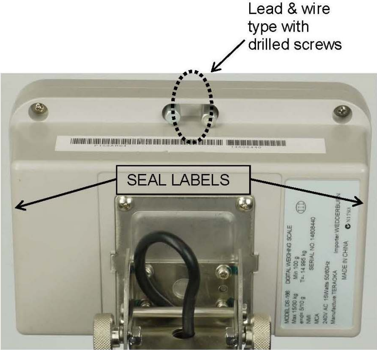
Typical Sealing Methods
