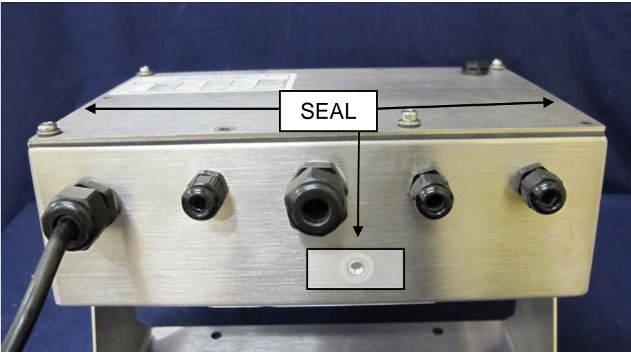
Typical Sealing Using Destructible Adhesive Labels
