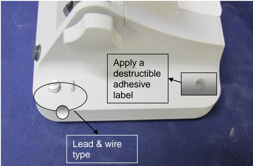
Typical Sealing of Mettler Toledo Model IND 231 Digital Indicator
