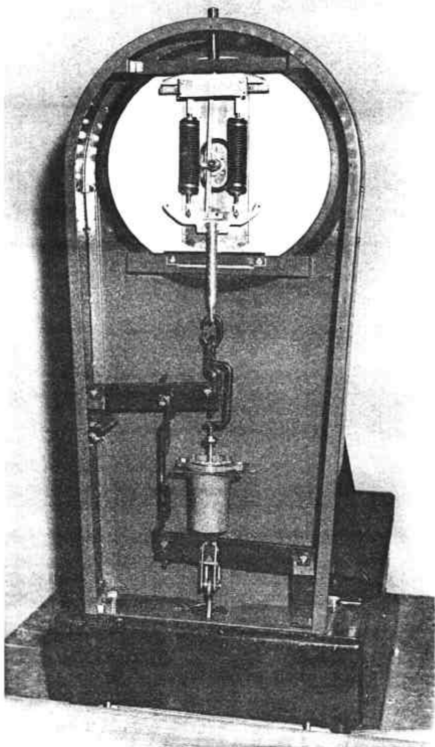
Avery 3552 CUB Weighing Instrument
