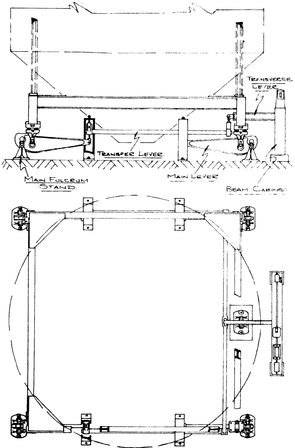
Howe Richardson Model SP-K (Printbeam) Grain Hopper Scale
