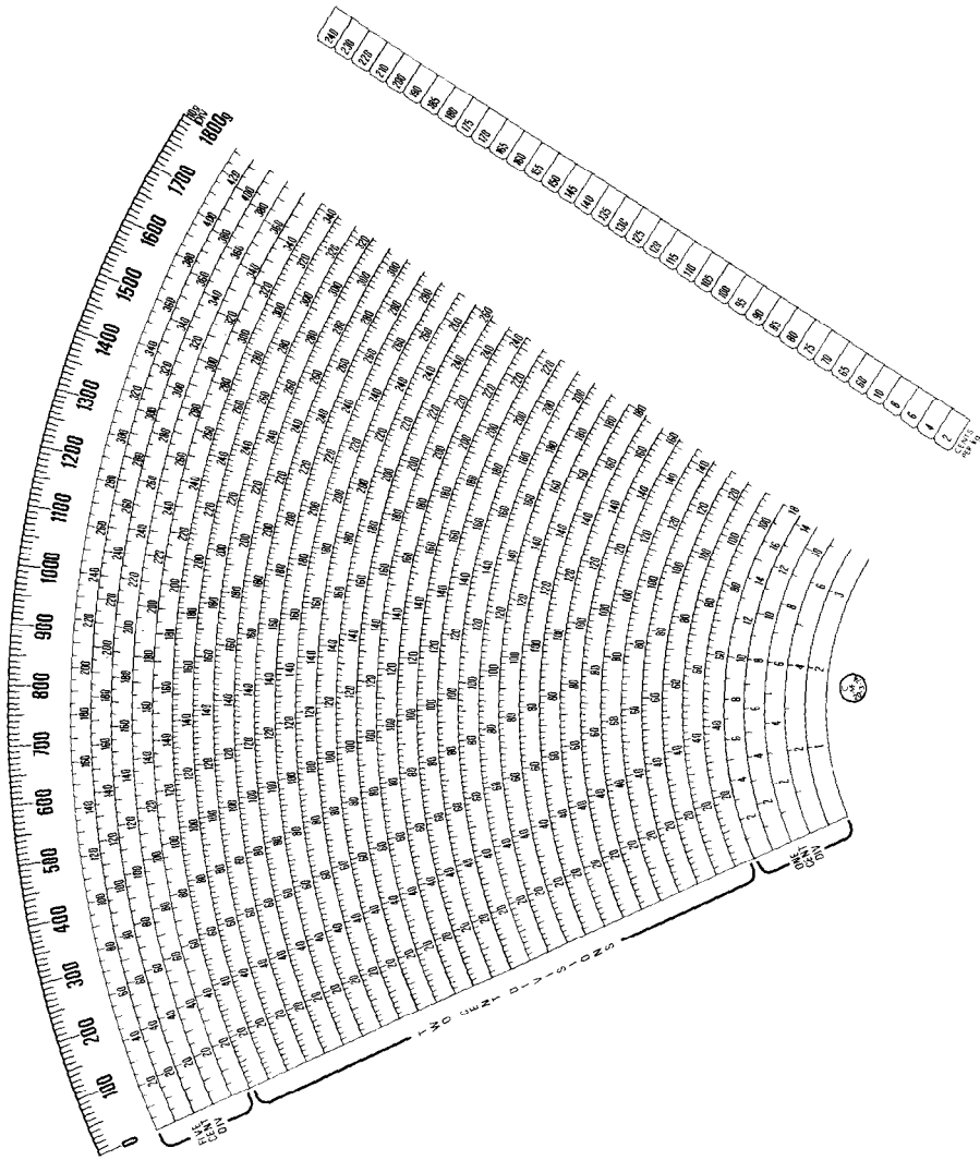
2-240-c/kg Chart and Indicator
