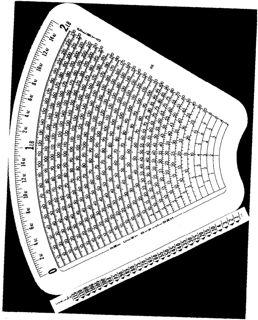
Chart H16 and Indicator H16
