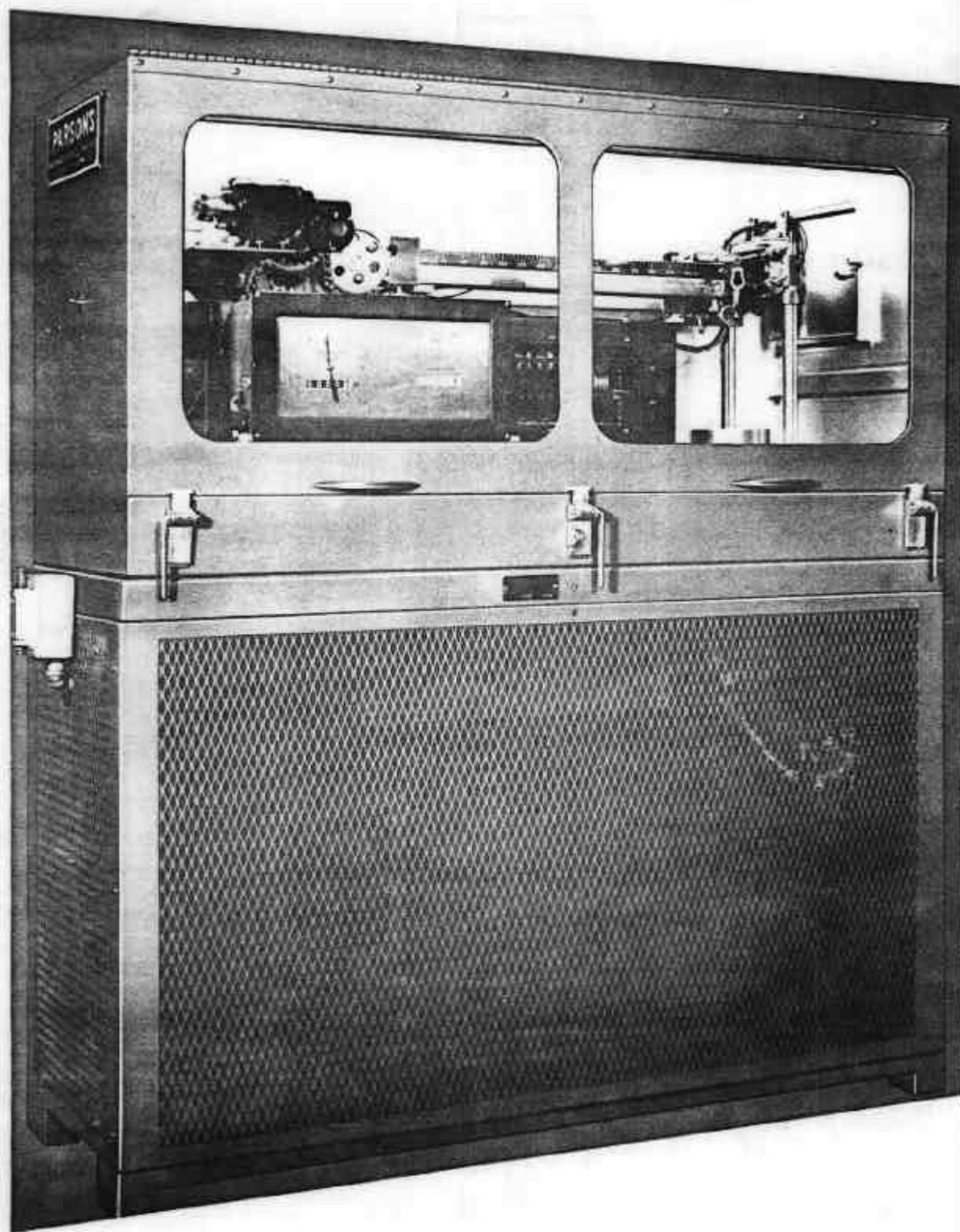
Parsons Hopper Weighing Instrument
