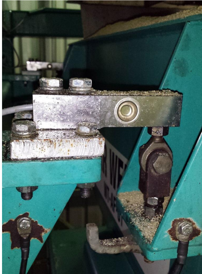
Load cell mounting
