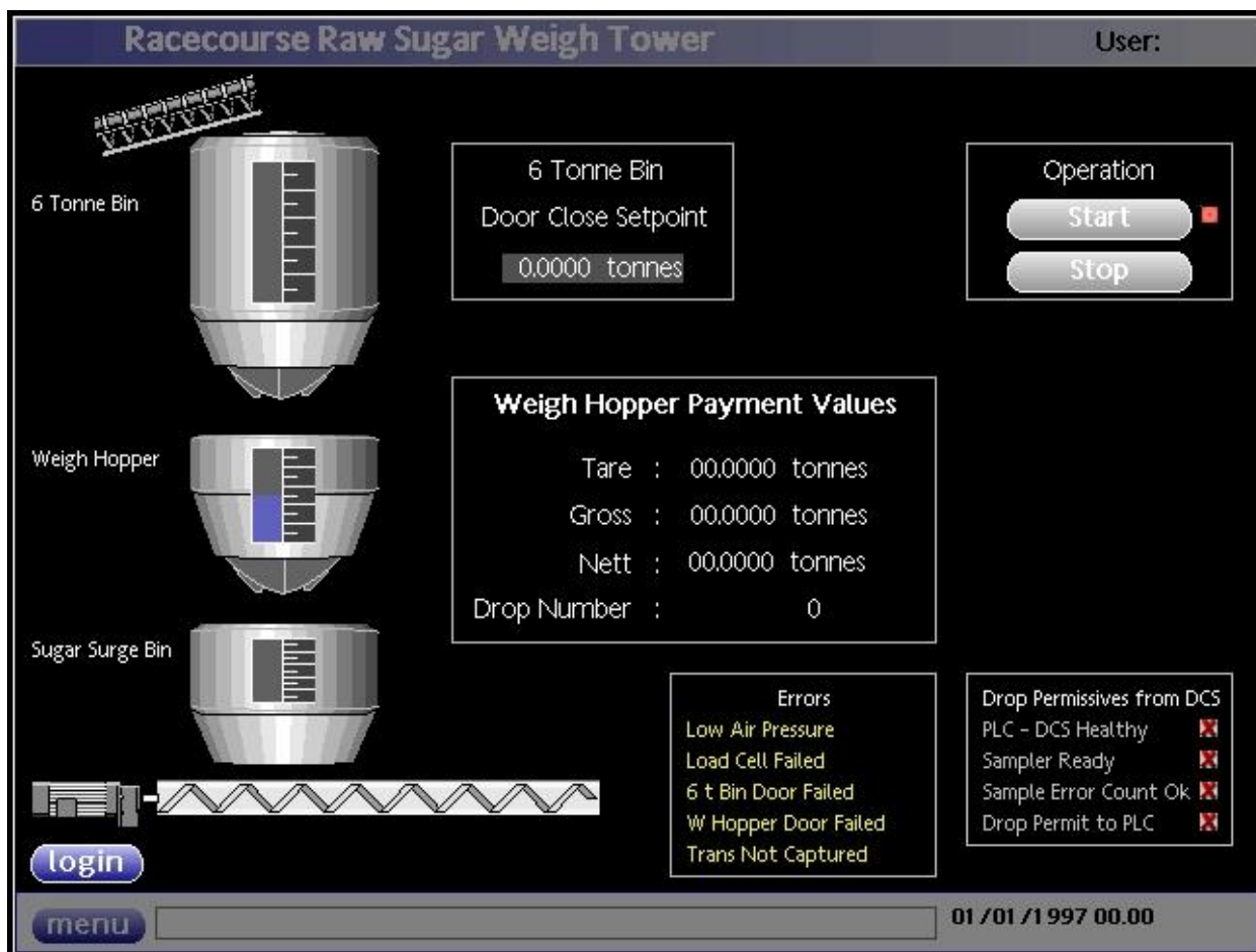
Accurate Systems Model AS-DT2 System Operator Screen (Typical example – screens may vary between installations)
