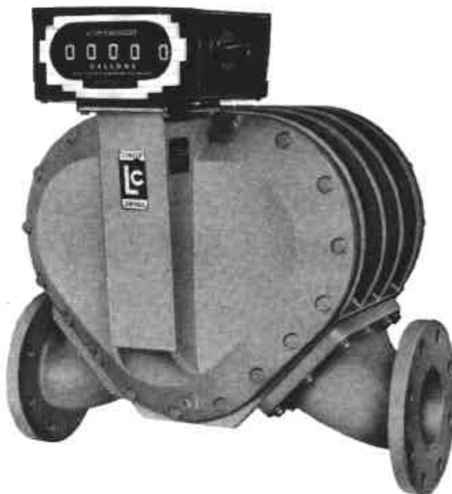
FIGURE 3. Liquid Controls Flowmeter Model M30
