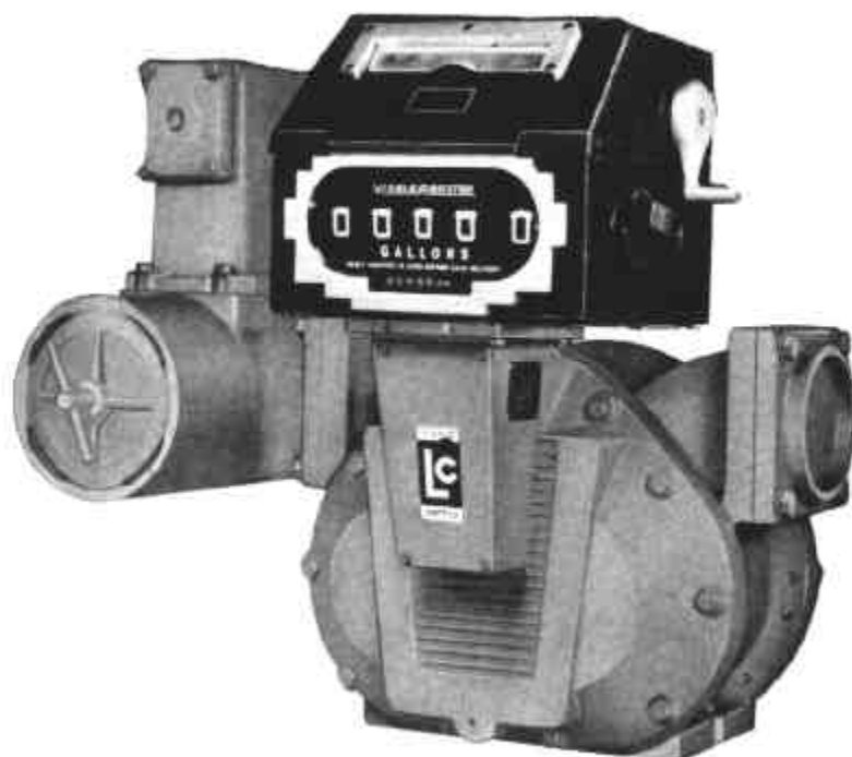
FIGURE 1. Liquid Controls Flowmeter Model M7
