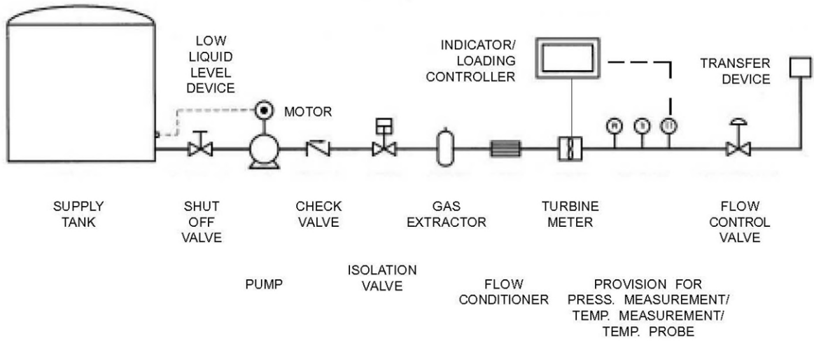
Typical Smith Meter Inc Turbine Horizontal Bulk Flowmetering System (The Pattern)
