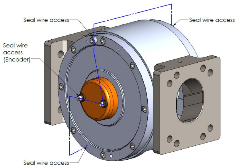
Compac COM 650 flowmeter (Variant 8)
