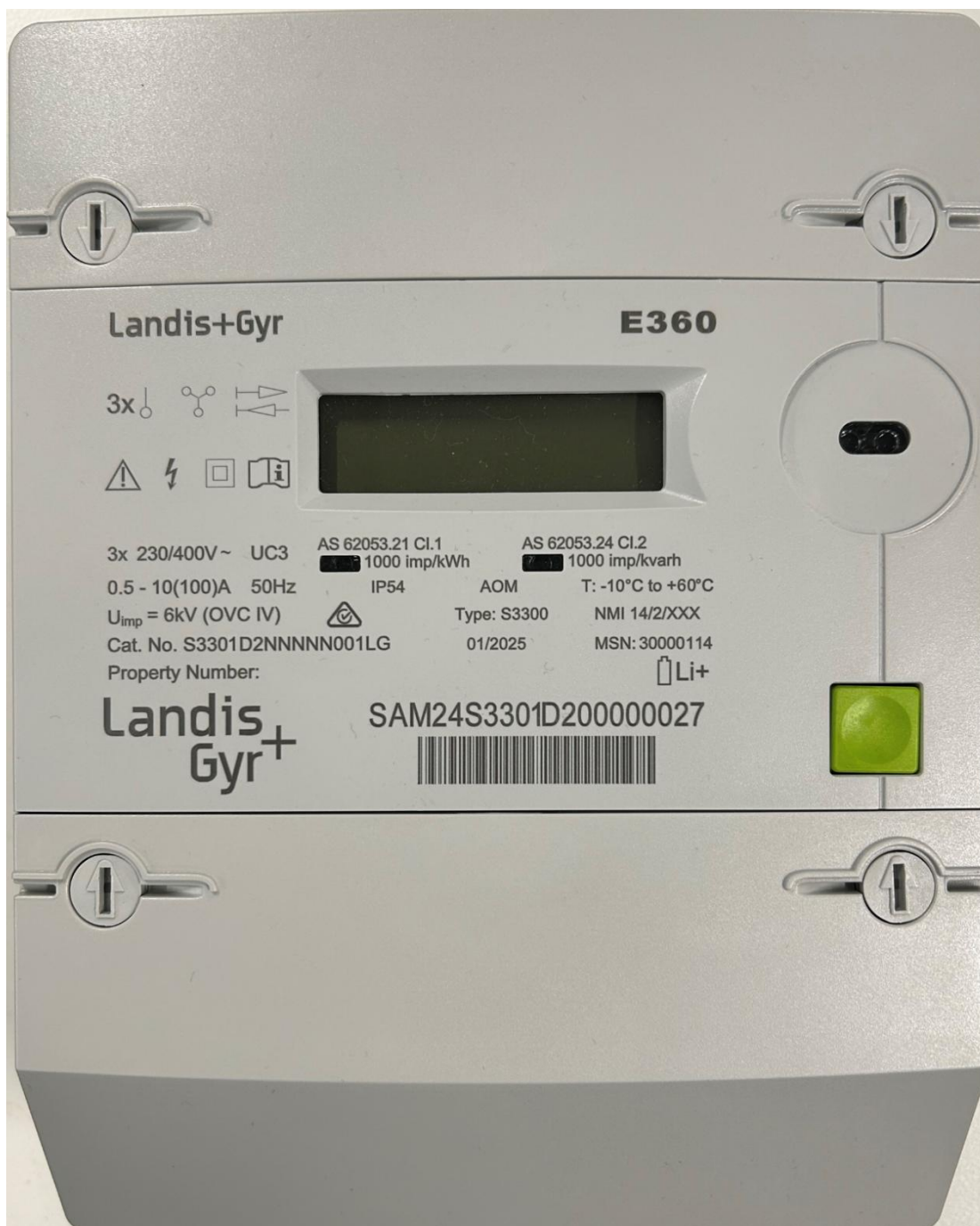
Landis+Gyr model E360 Type S3301 Electricity Meter (Variant 6)
