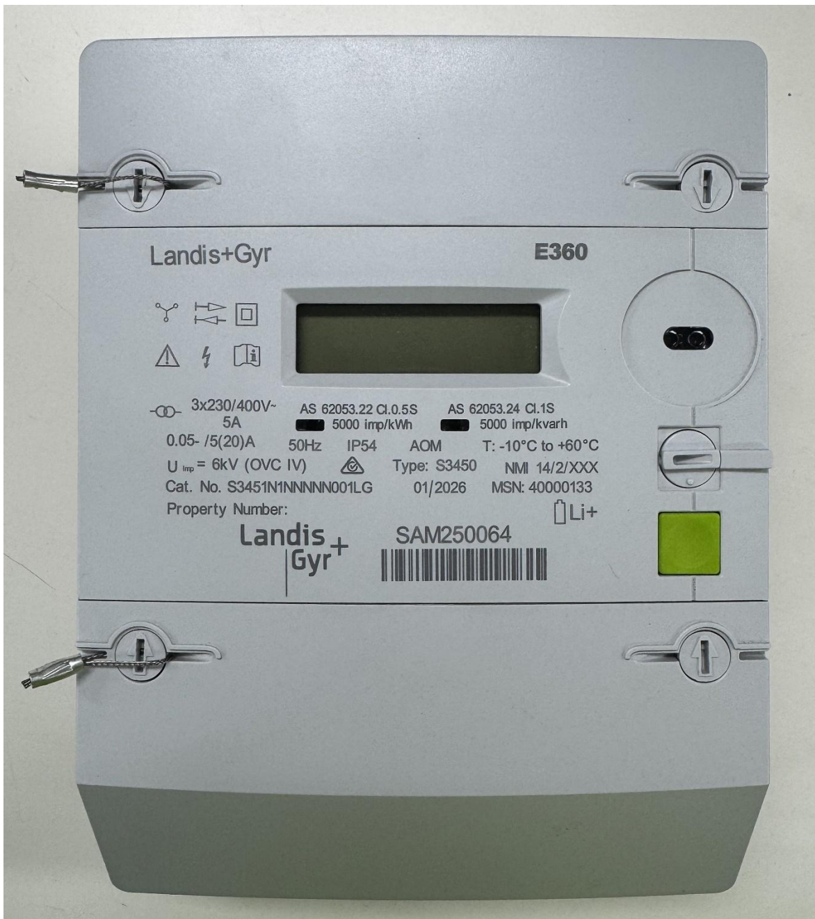
Landis & Gyr Pty Ltd model E360 Type S3450 Electricity Meter with 230 V (The Pattern, Including Typical Mechanical Sealing)
