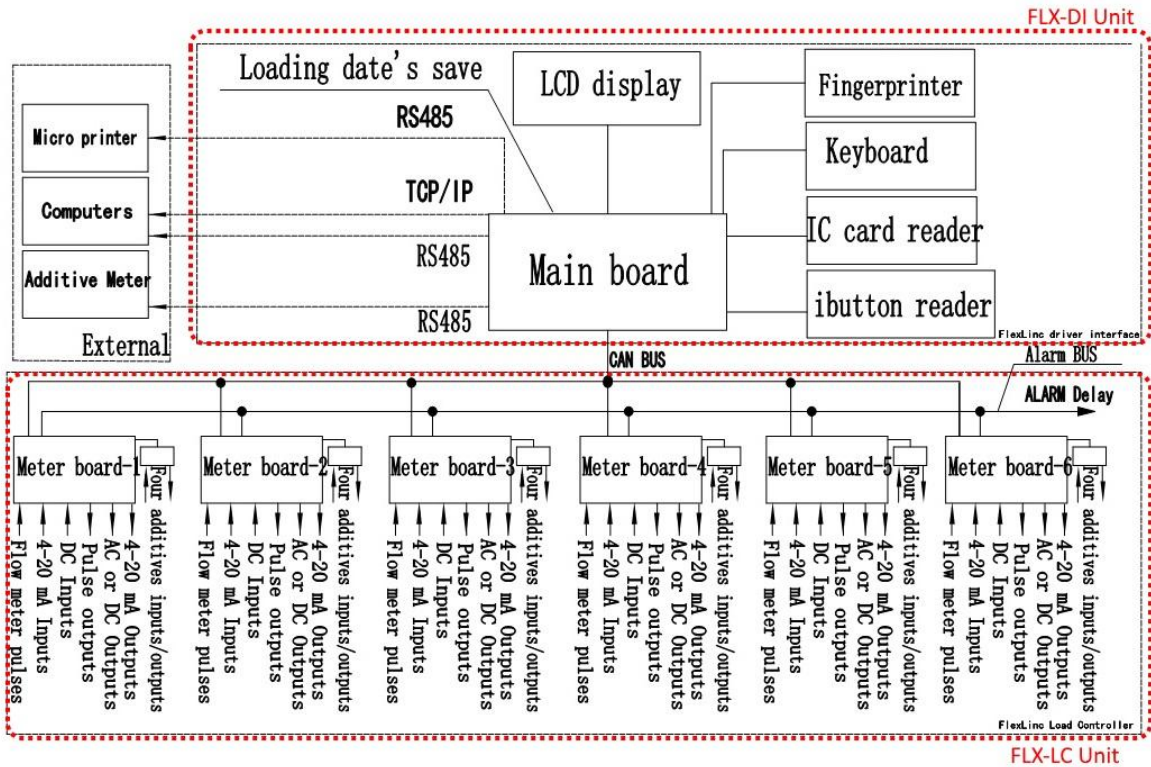
FlexLinc Model FLX-BC Controller System in Separate Housings (Variant 1)
