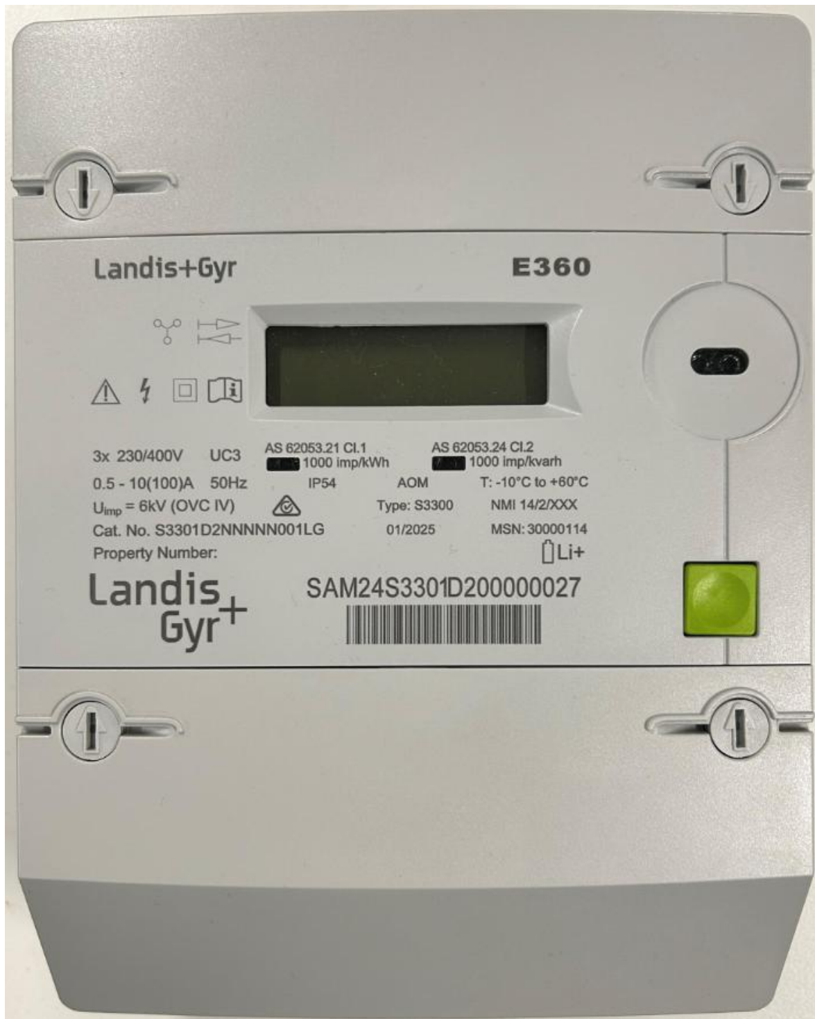
Landis+Gyr Pty Ltd model E360 Type S3301 Electricity Meter (Variant 4)
