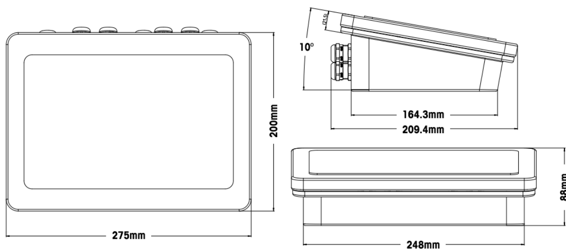
Mettler Toledo Model IND360 Harsh Version and Sealing Method (Variant 2)
