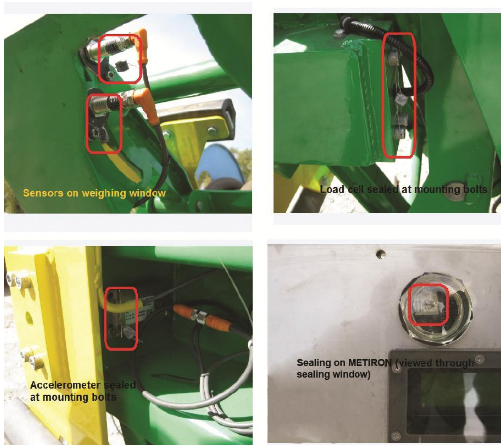
Sealing Arrangements
