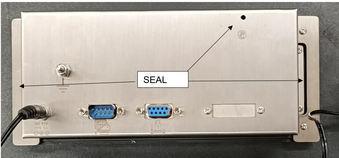
Sealing of Model BM1000P Painel Typical Sealing Methods
