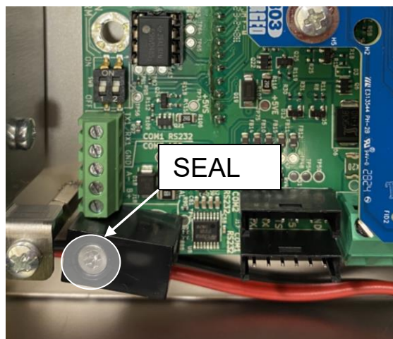
Typical Sealing of Protective Cover (New Mainboard)
