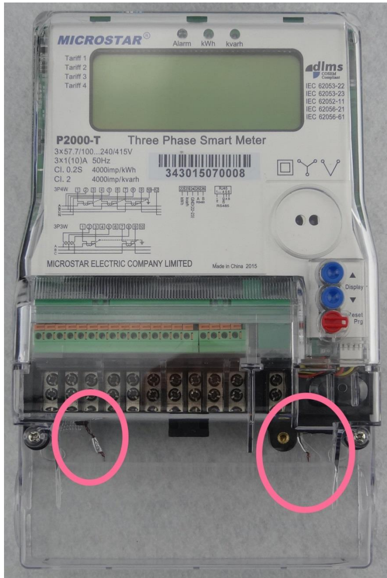
Microstar Model P2000-T (Including Typical Mechanical Sealing)
