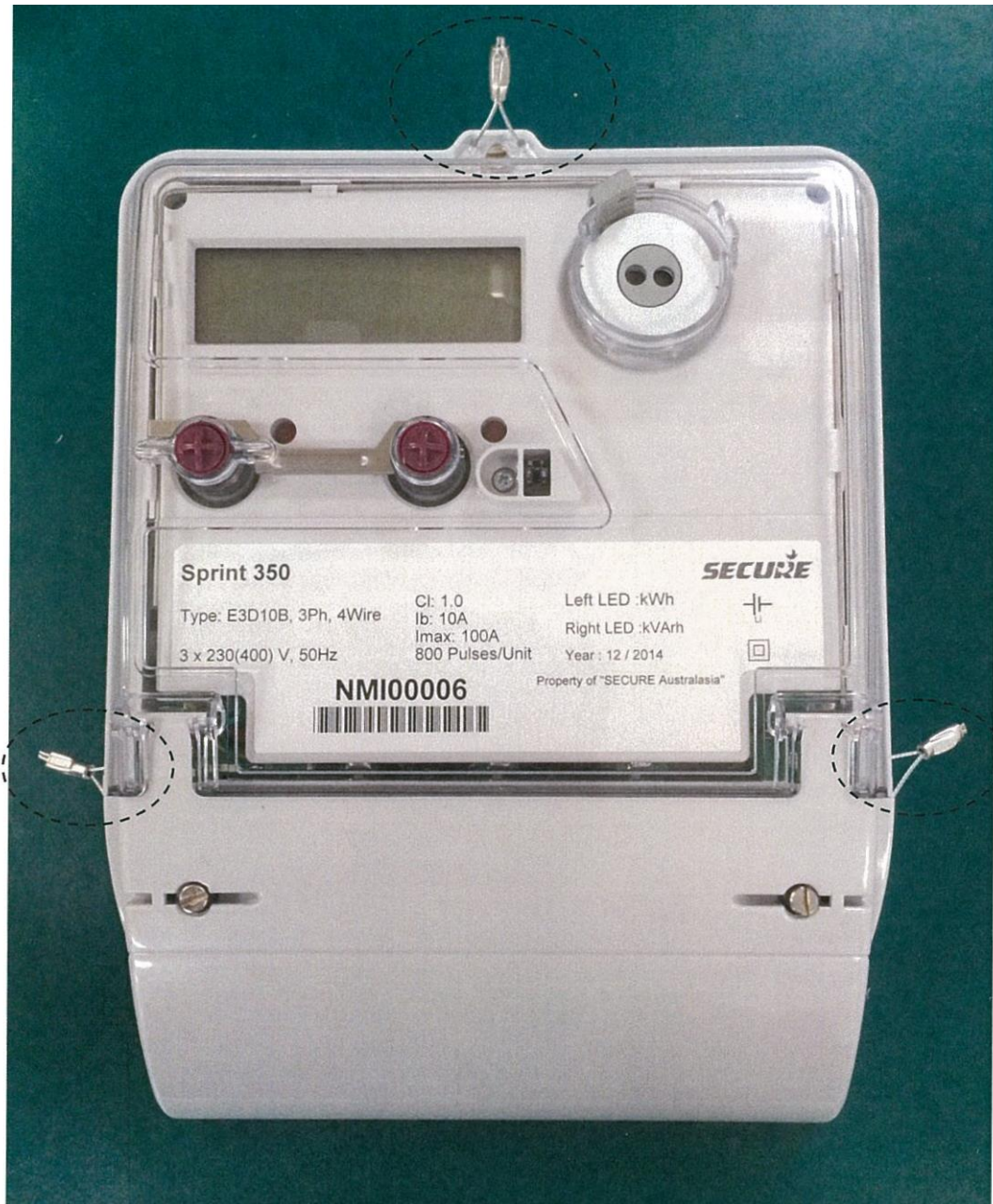
Typical Mechanical Sealing
