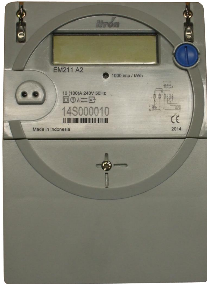
Itron Australasia Model EM211-A2 (Including Provision for Mechanical Sealing)
