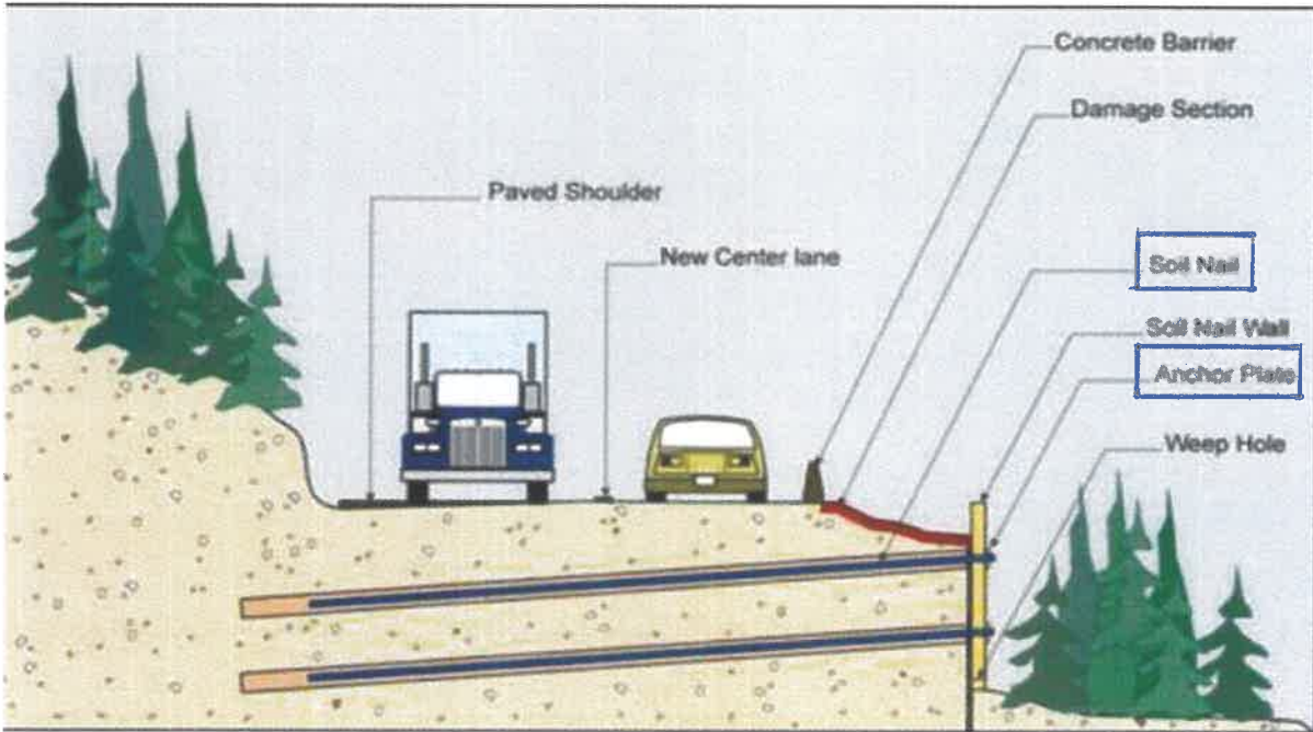
Figure 1. Soil Stabilisation using 500N Bar example
