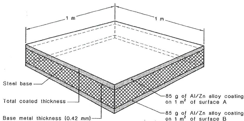
FIGURE C1 COATING MASS ILLUSTRATION (NOMINAL 150 g/m 2 OF SHEET)
