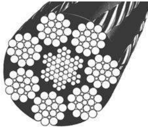
Plastic coated wire rope construction.
