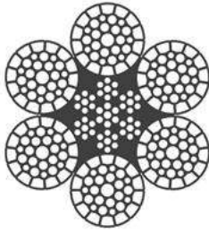
Plastic impregnated wire rope construction.
