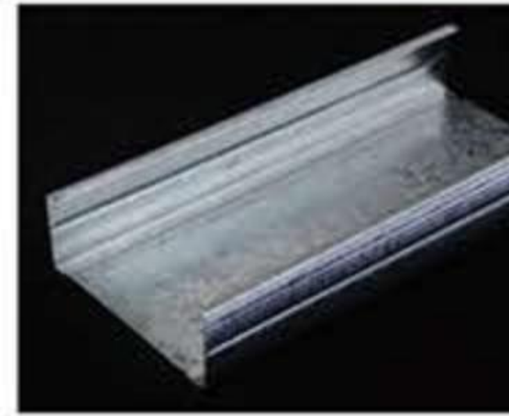
Metal Stud 51x33.5x35.5x3000 0.55BMT 0.554kg 64x33.5x35.5x3000 0.55BMT 0.609kg 76x33.5x35.5x3000 0.55BMT 0.599kg 92x33.5x35.5x3000 0.55BMT 0.732kg
