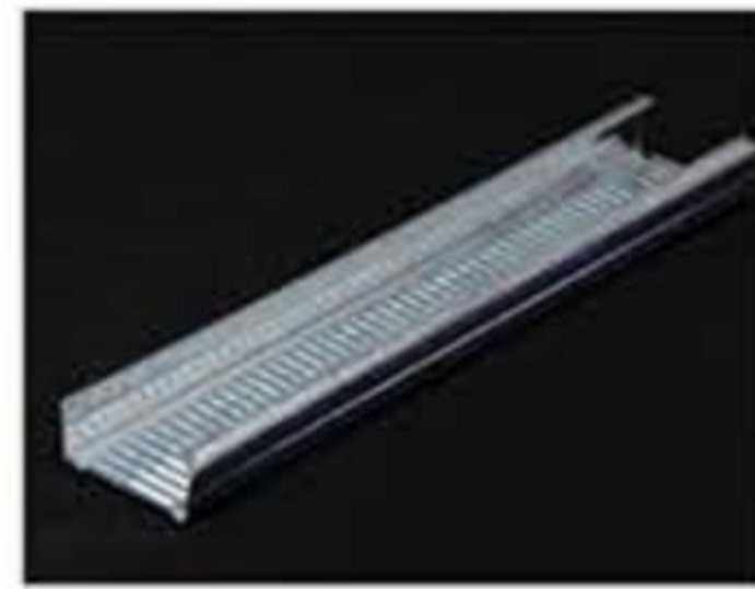
16 Ceiling Batten 36x16x6000/4800mm 0.50 BMT 0.291kg plm
