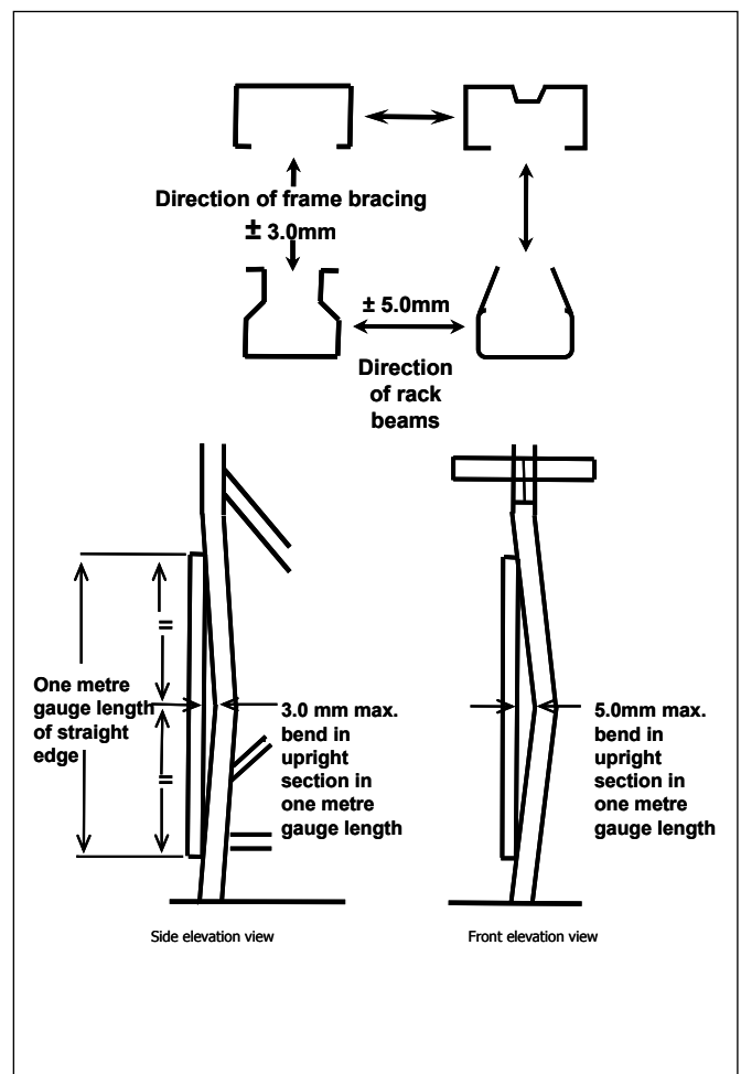
Figure 4: Typical upright sections and method of measurement
