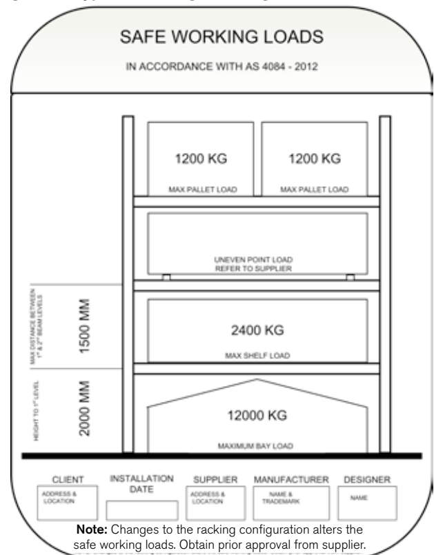
Figure 1: Typical racking SWL sign
