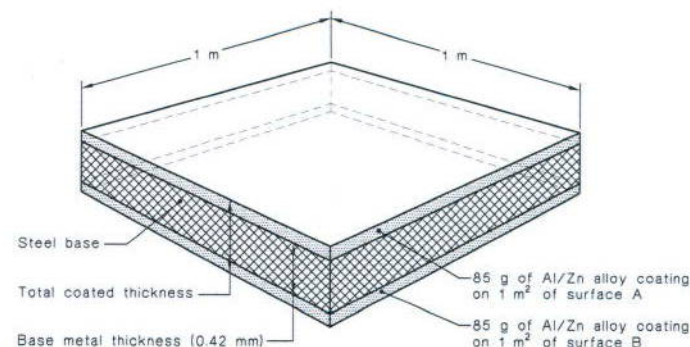
FIGURE C1 COATING MASS ILLUSTRATION (NOMINAL 150 g/m 2 OF SHEET)
