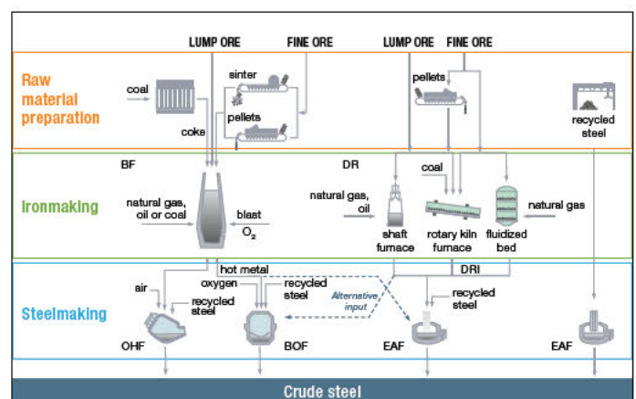
Figure 2: Steelmaking routes
