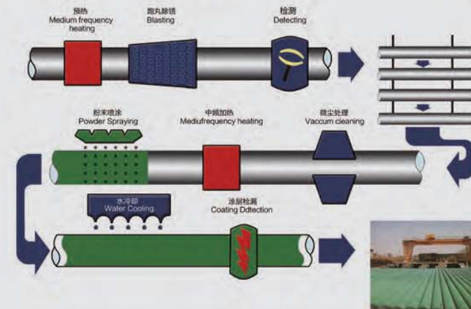
2PE/PP、3PE/PP涂敷工艺流程示意图 Process Diagram of 2PE/PP、3PE/PP Coating
