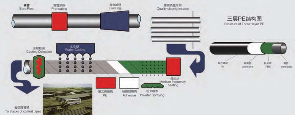
2PE/PP、3PE/PP涂敷工艺流程示意图 Process Diagram of 2PE/PP、3PE/PP Coating
