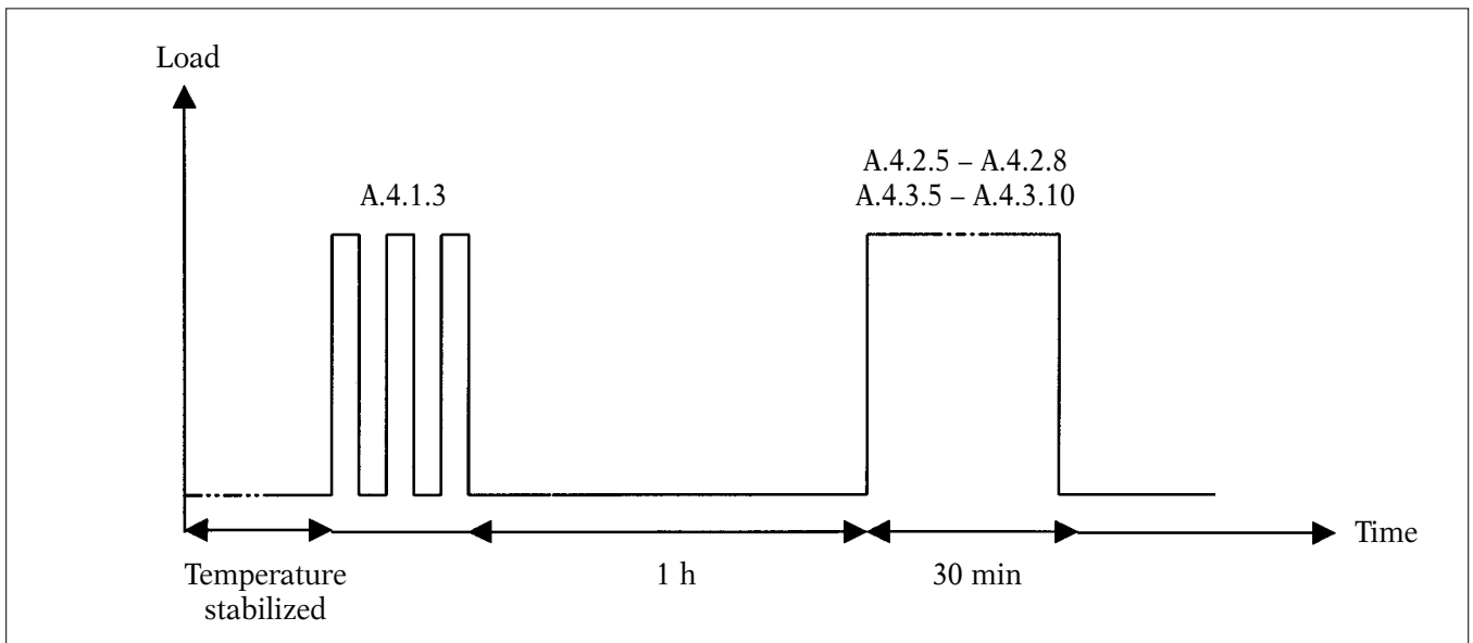
Figure A.2 Recommended test sequence for each test temperature for the minimum dead load output return (DR) and creep tests when carried out in a machine different from that used for the load tests
